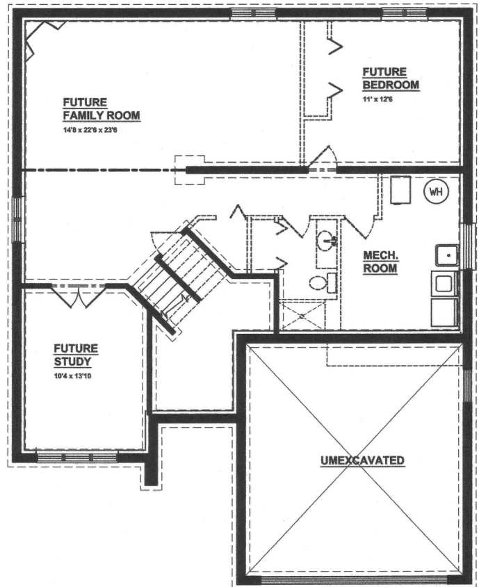
FOUNDATION PLAN
